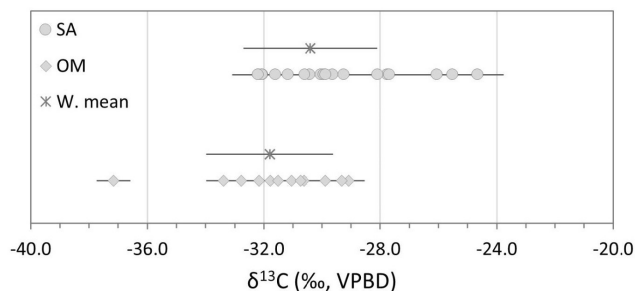
FIGURE 7 In situ carbon isotope results from nodular black chert samples (NBC texture 3 of Barlow, 2019; Barlow & Van Kranendonk, 2018). SA microfossil data are depicted by circles (asterisk above SA data set is w. mean: \delta^{13}\text{C} -30.4 \pm 2.3\% ; n = 19 ). Data collected from the dense and fluffy OM were combined and are displayed here as diamonds (asterisk above OM data set is w. mean: \delta^{13}\text{C} -31.8 \pm 2.2\% ; n = 12 ). For definition of w. mean, see Table S1. Grey bars in main data sets indicate error (for individual measurement errors, see Tables S2–S4). Grey bars for weighted means = 1SD.
