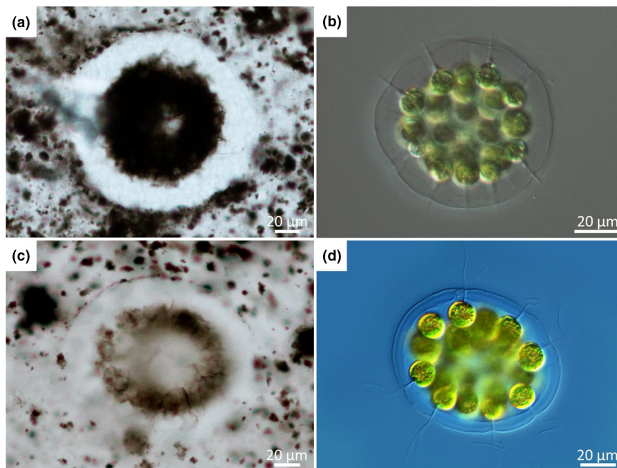
FIGURE 10 Direct comparison of Turee Creek Group SA microfossils (a, c) and extant, Volvocacean coenobial algae (Eudorina; b, d). Note similarities in symmetrical shape, structure and overall size. Spherical (a) and ellipsoidal (c) microfossils with wide, kerogen-free rinds; PPL. Compare with spherical (b) and ellipsoidal (d) coenobia that are surrounded by thick, clear, extracellular mucilage. Also note the thin, wire-like structures and apparent hollow centre of the microfossil in part (c) (and the hint of a hollow centre within the specimen in part a) and compare with the flagella and hollow centre of the coenobia in parts (b) and (d). Image credit: (b) Matthews (2016) and (d) Antonio Guillén.
