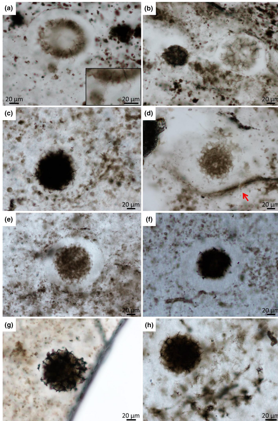
FIGURE 3 In thinner (~30 \mu\text{m} thick) petrographic sections, SA microfossils are more transparent, revealing an internal framework of honeycomb-like compartments. The compartments are sub-spherical to polygonal in shape and are composed of dark brown, often granular, OM. (a) SA specimen with a hollow core and an even rind that is partially outlined along the outer, top edge. Inset shows enlarged view of thin, wispy structures emanating out from the SA body into the surrounding rind. (b–h) Variably preserved SA microfossils and surrounding rinds. Arrow in (d) points to deflected underlying bedding (see also Figure S7 ). Fragments of thick filamentous microfossils are visible in (f) and (h). The line in (g) that cuts diagonally across the image is the broken edge of the thin section. All images are vertical cross sections through bedding in PPL.
