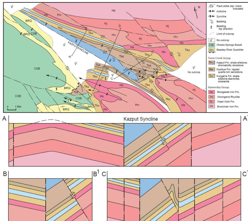
Fig. 2 Detailed geological map of the study area, showing the Kazput Formation stromatolitic dolostone in darker blue. This unit forms the eastern limb of the north-west plunging Kazput Syncline, the axial trace of which is marked by a fault (above 'Kazput Syncline' label). Lines A–A 1 , B–B 1 and C–C 1 denote the location of the cross sections, which are drawn at an expanded scale compared to the map, but with the vertical scale equal to the horizontal scale.
