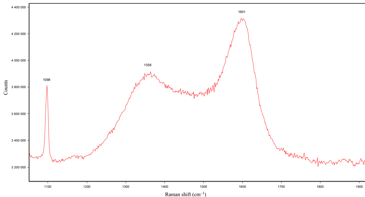
Fig. 18 Columnar stromatolite Raman spectrum exhibiting peaks characteristic of kerogen: the disorder or 'D' band (Castiglioni et al. , 2001) centred at \sim 1358\text{ cm}^{-1} and the graphitic, or 'G' band (Tuinstra & Koenig, 1970) centred at \sim 1601\text{ cm}^{-1} . Note the carbonate peak centred at \sim 1098\text{ cm}^{-1} .
